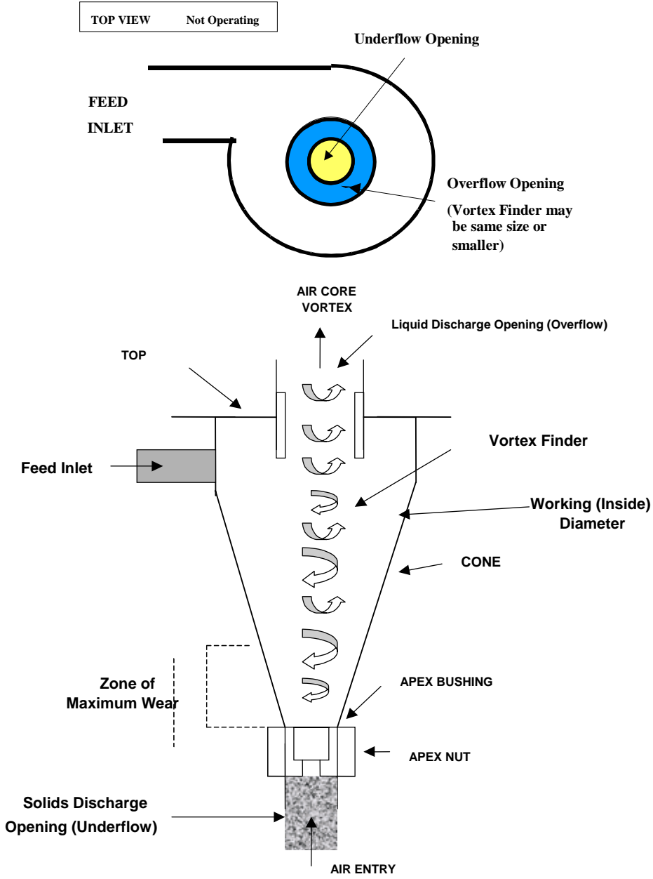
Drawing: Spray Discharge of Hydro cyclone
