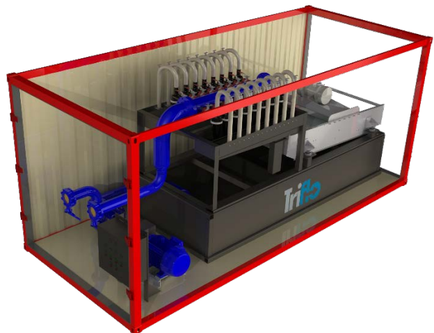
Removable Equipment Skid for De-Sanding Unit for Non Routine Maintenance
