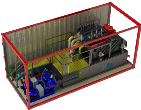
Three Phase Cleaning at 120 GPM, Hopper Can Be Added for Small Batch Mud Treatment
