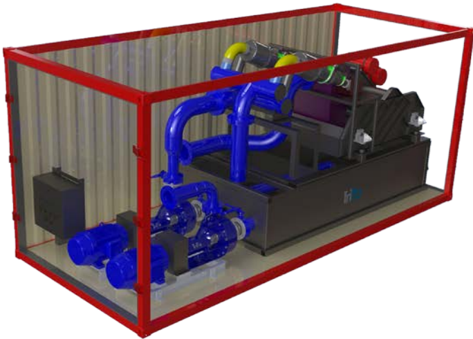
Two Phase, 1000 GPM De-Sanding Unit
